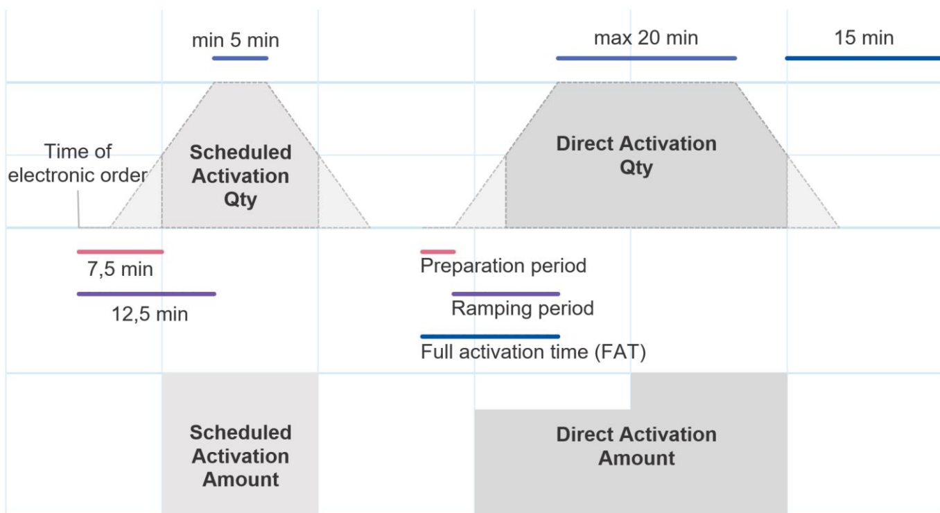
Figure 15. Ramping of volumes on mFRR activations over three or four imbalance settlement periods.
